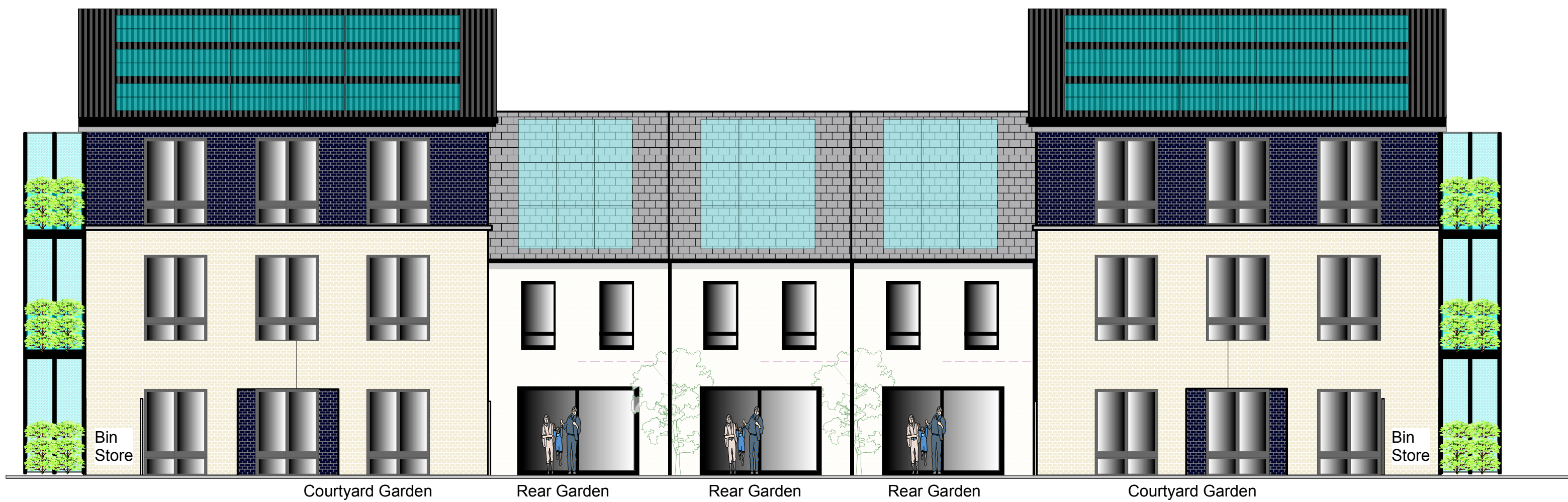
South Section & Internal Elevations
