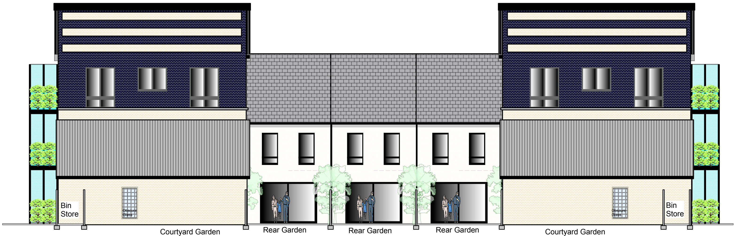
North Townhouse 2 Elevations & Internal Elevations
