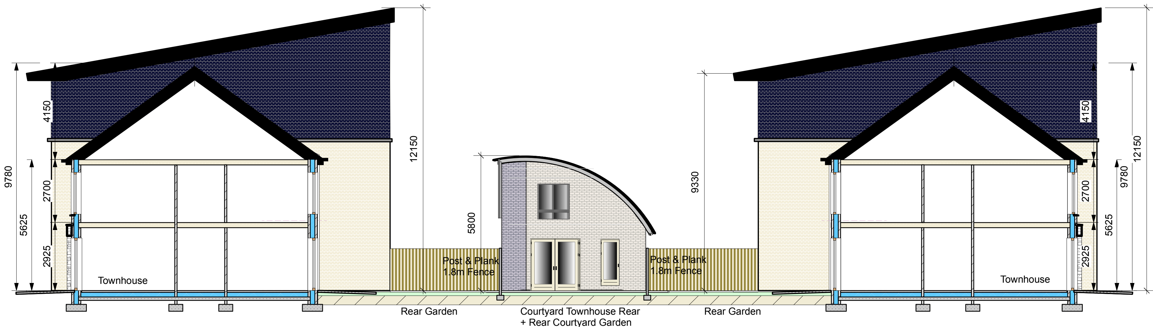
West Facing Cross-Section & Internal Elevations
