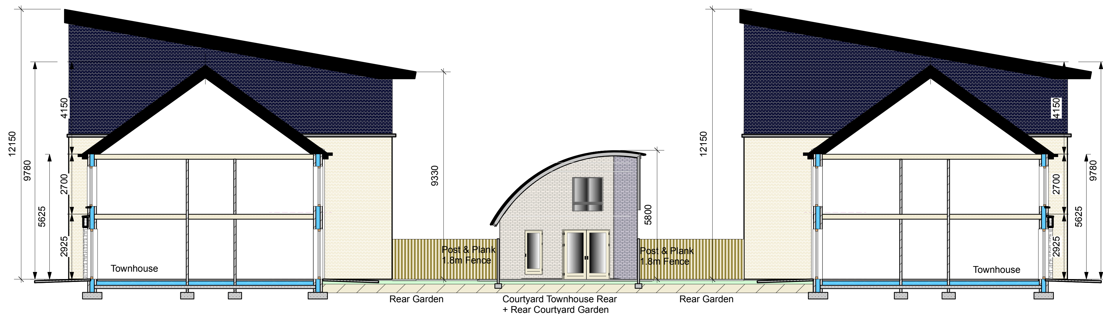
East Facing Cross-Section & Internal Elevations
